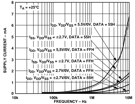
Figure 13. Supply Current vs. Clock Frequency
